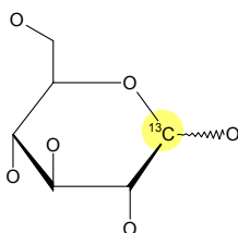
D-Glucose-1-13C
