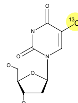
Thymidine, methyl-13C
