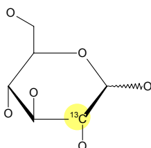
D-Glucose-2-13C
