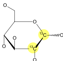
D-Glucose-1,2-13C2
